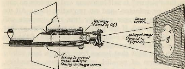
THE EYEPIECE AS AN ENLARGING LENS—Observing the Sun by projection
