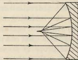
Spherical Aberration—uncorrected spherical mirror.
