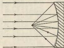
Spherical Aberration eliminated by "figuring" mirror to paraboloidal form.
