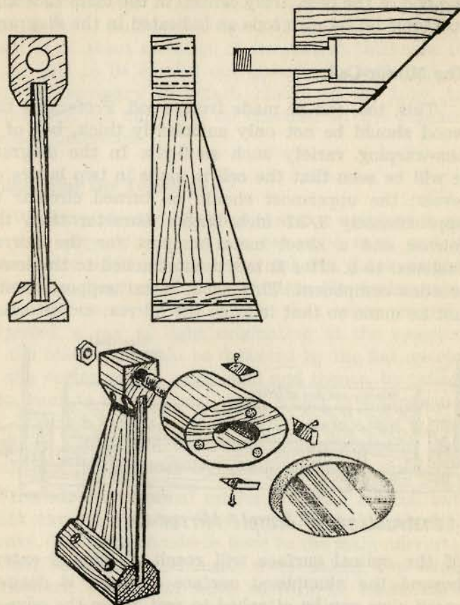
Mounting the Newtonian Flat
