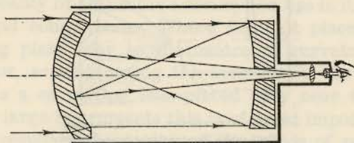
Maksutov-Gregorian Telescope
