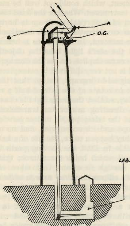
TOWER-TELESCOPE: THE SUN'S LIGHT IS CONSTANTLY DIRECTED VIA THE HELIOSTAT (A) AND DIRECTING MIRROR (B) INTO THE OBJECT-GLASS (O.G.). THE IMAGE IS FOCUSED BELOW GROUND VIA THE FLAT AT THE BOTTOM OF THE SHAFT. THE HELIOSTAT IS EQUATORIALLY MOUNTED AND IS DRIVEN AT RATE OF \frac{1}{2} rev p. day.
