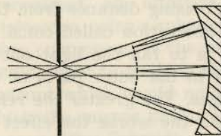
Spherical Mirror + Small Stop at Centre of Curvature; Wide-field, coma-free, curved focal surface—low photographic-speed.
